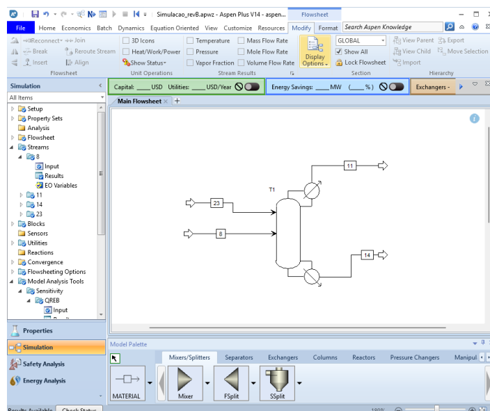
Figura 1: Fluxograma configurado no Aspen Plus
